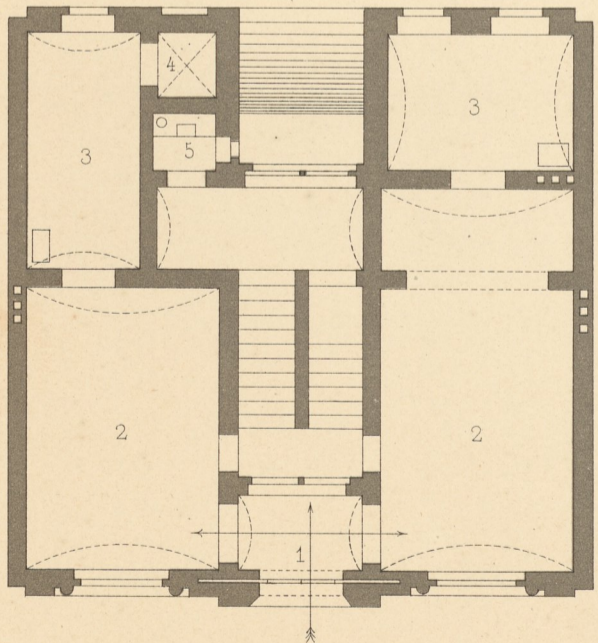
Erdgeschoss.
