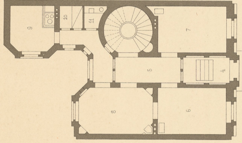
Erdgeschoss.
