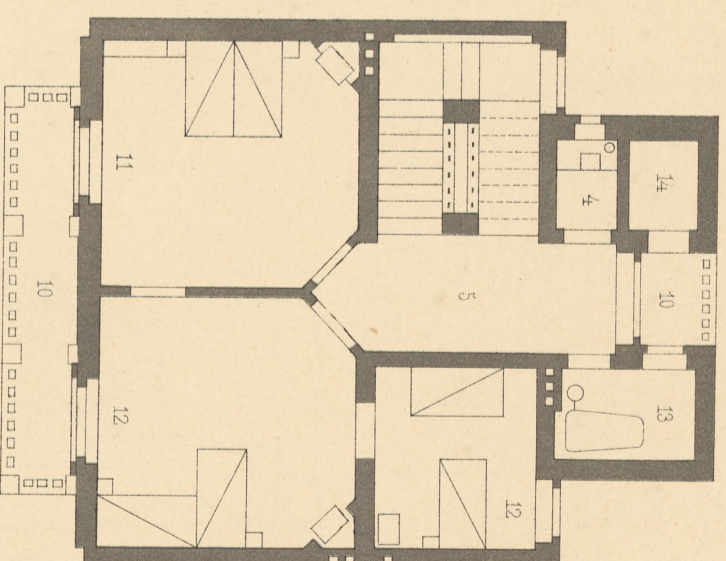
II.ter Stock.
