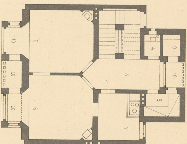
I.ter Stock.
