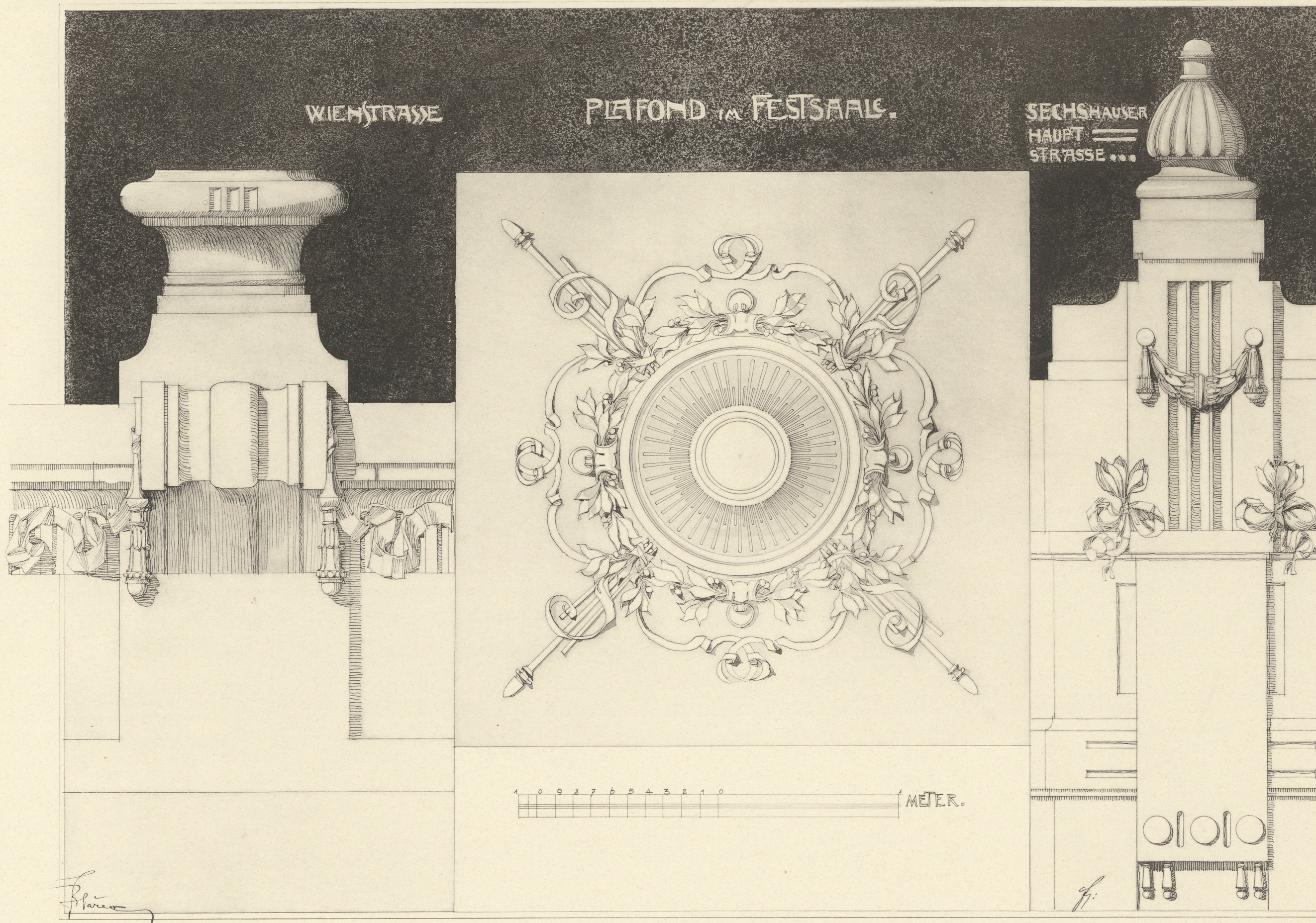
FAÇADENDETAIL.
