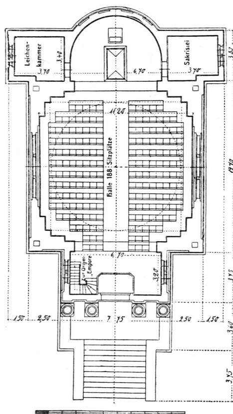
Erdgechofs.
