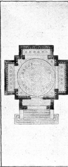
Erdgechofs.
