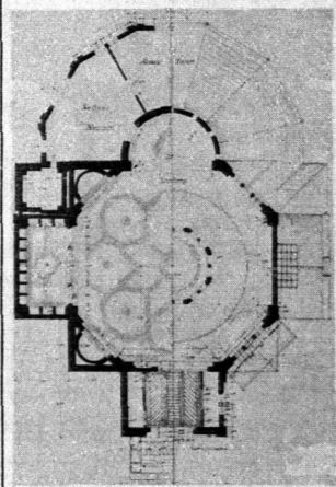
Fig. 260. Erdgeschofs.
