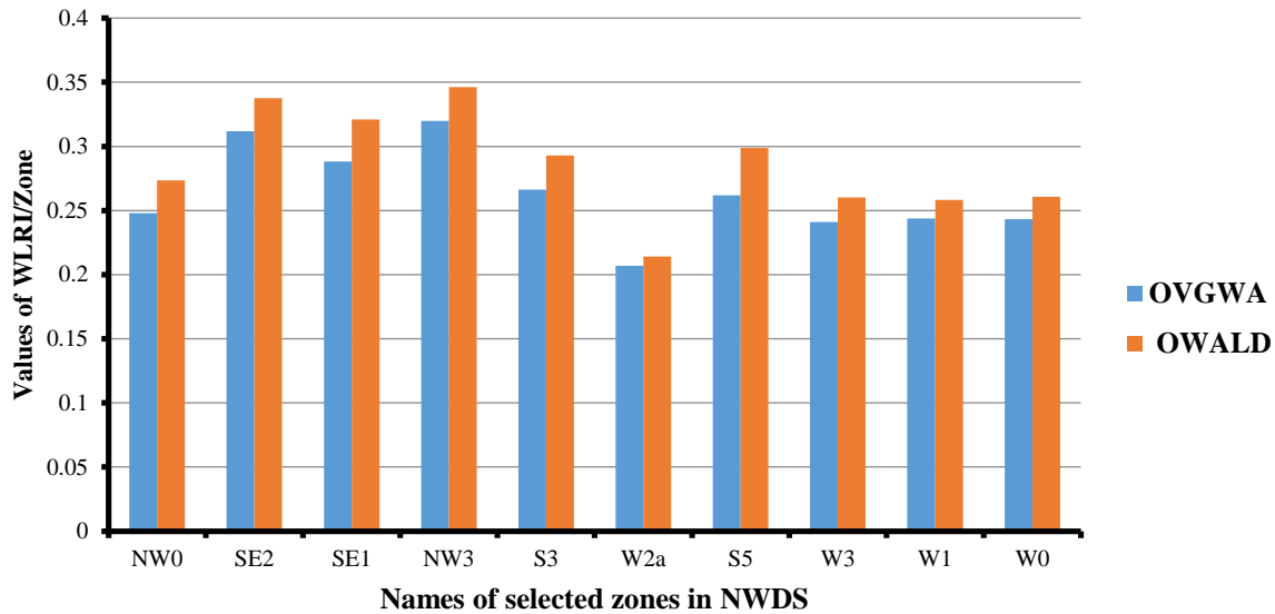
Figure 39. Illustration of values of WLRI/ Zone generated by OVGWA and OWALD aggregation techniques.
