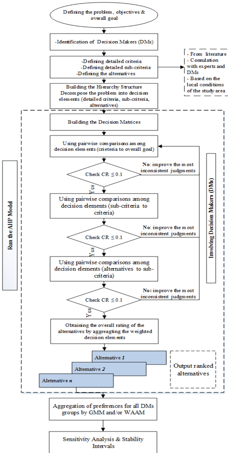
Figure 9. Flowchart of AHP method used to build a water loss management framework.
