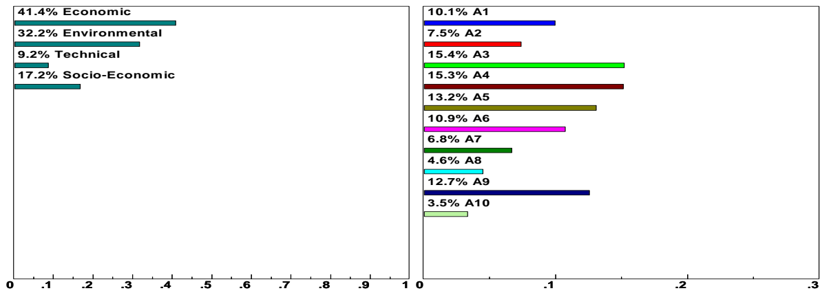
Figure E3 | Dynamic sensitivity analysis for environmental criterion – maximum limit of stability interval.
