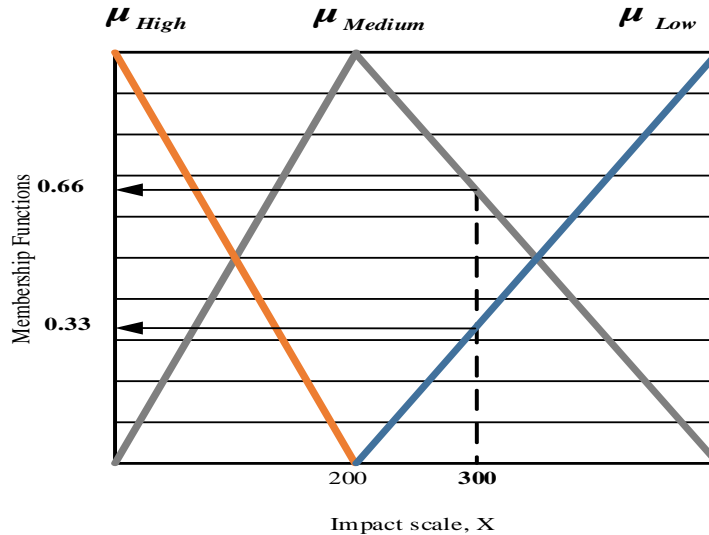
Figure 15. Membership functions and fuzzification of pipe diameter contributed to WLRI as an example.
