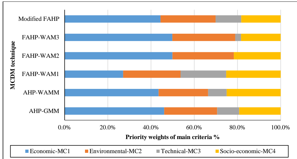
Figure 22. Distribution of weights of main criteria.
