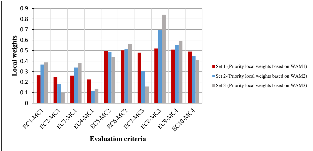
Figure 30. Local weights of evaluation criteria (Three sets) generated by Fuzzy AHP technique based on using three different weighted aggregation methods of DMs' evaluations (WAM1, WAM2 and WAM3).
