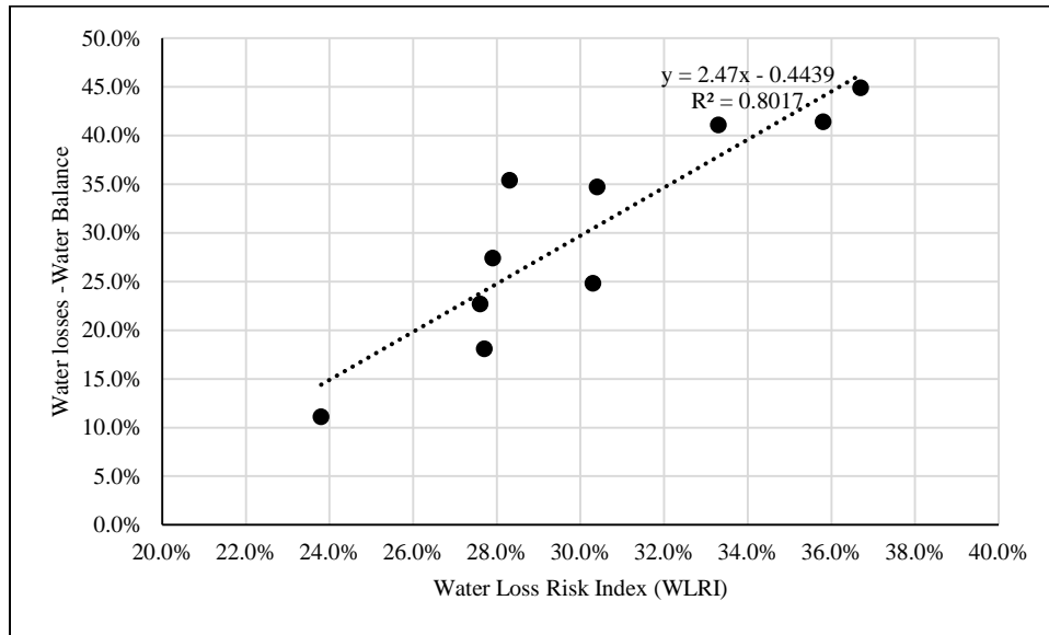
Figure 44. Correlation between water loss risk index (WLRI) of ten selected zones in NWDN and their total water losses from water balance calculations.
