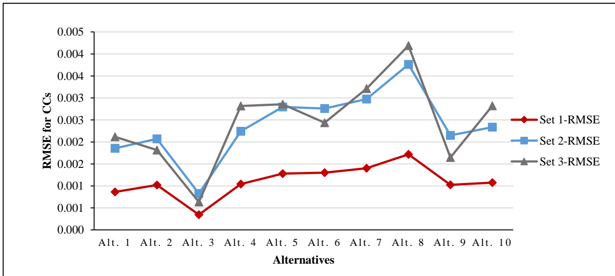
Figure 36. RMSE for CCs produced by sensitivity analysis with respect to the base condition (Set 1; the calculations of RMSE in association with the use of WAM1 method in Fuzzy AHP, Set 2; the calculations of RMSE
