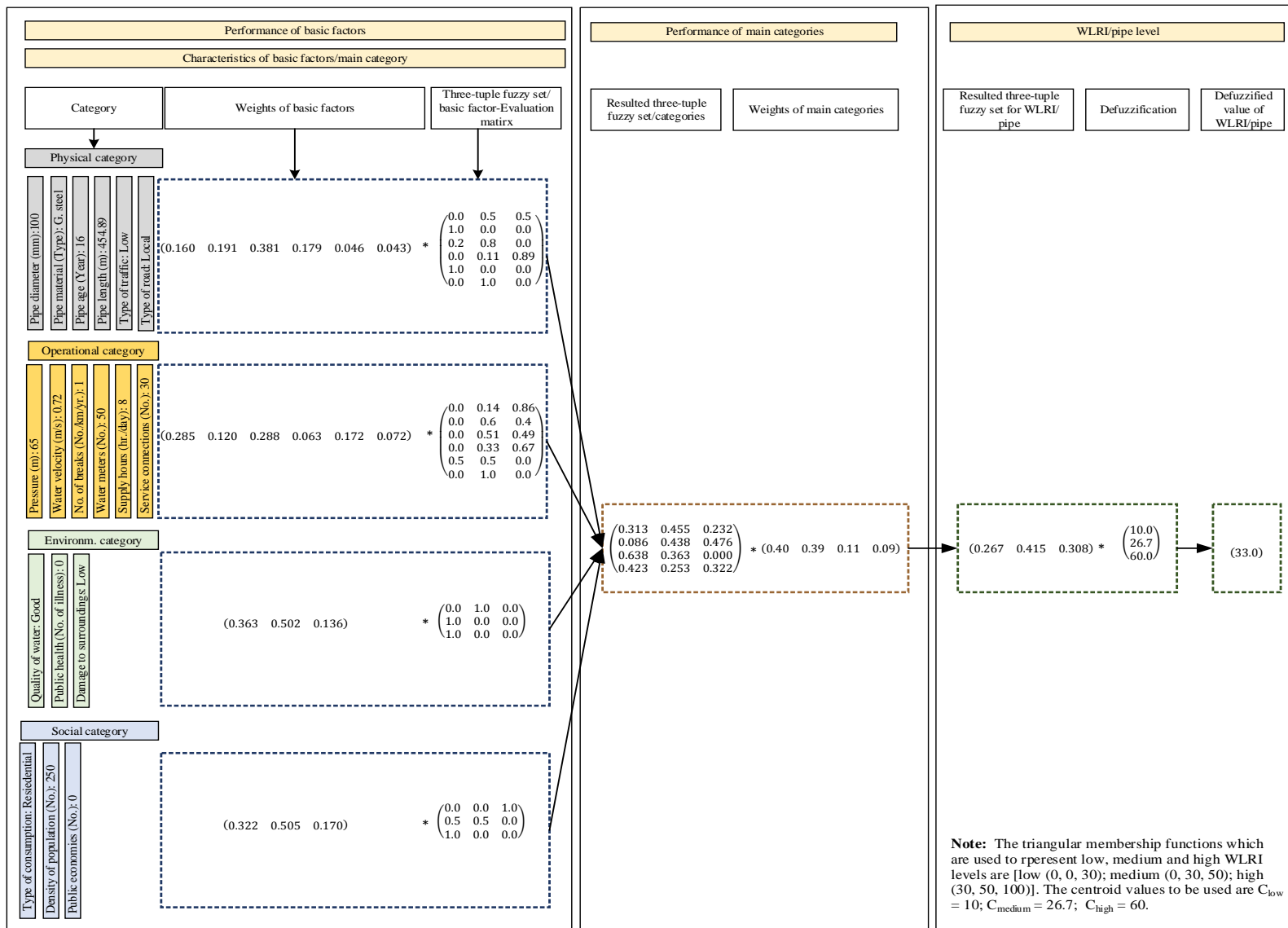
Figure 37. Sample of generating WLRI for a pipe with an ID 2085, Zone W0 -NWDS by FSE technique with the following some major characteristics: pipe diameter (100 mm), pipe material (Galvanized steel), pipe age (16 years), pipe length (454.89 m) and average pressure (65 m).
