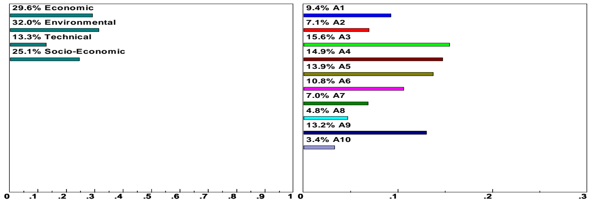
Figure E2 | Dynamic sensitivity analysis for economic criterion – minimum limit of stability interval.
