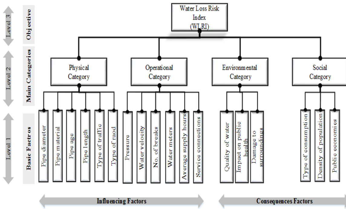
Figure C.1 Hierarchical structure of contributing factors to water loss risk index (WLRI) in water distribution networks.
