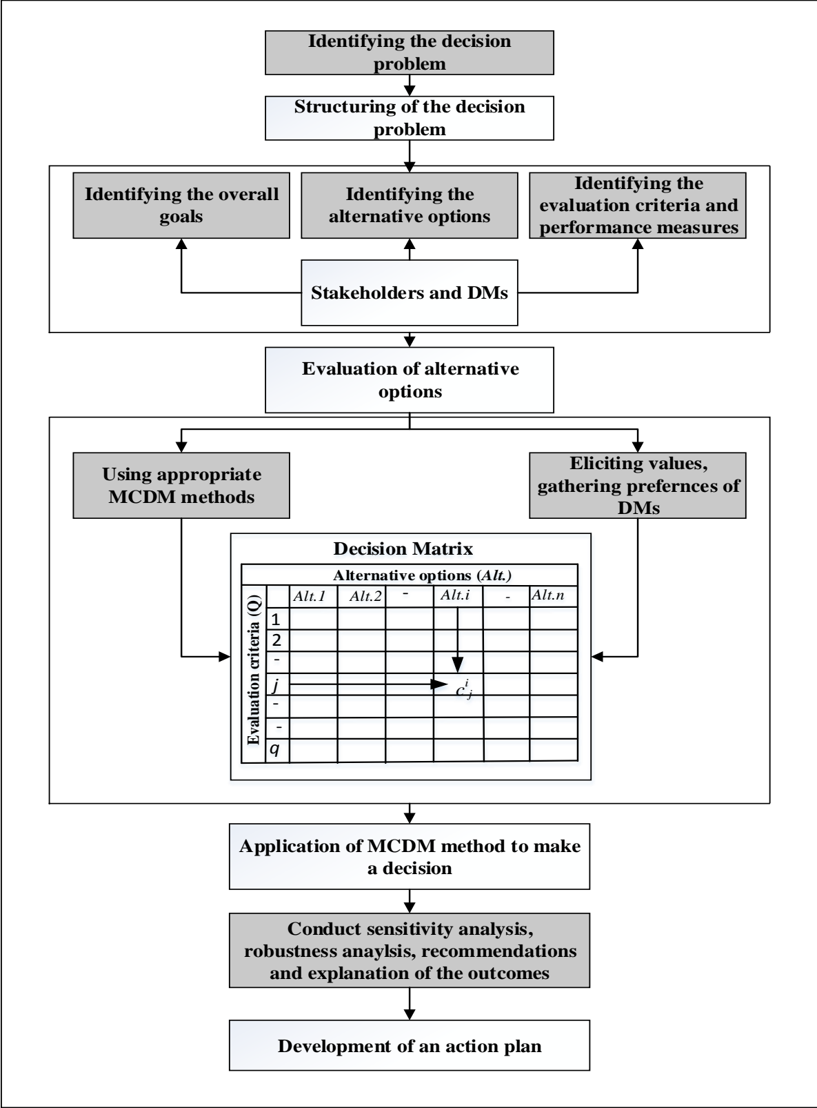
Figure 6. General steps in an MCDM process.
