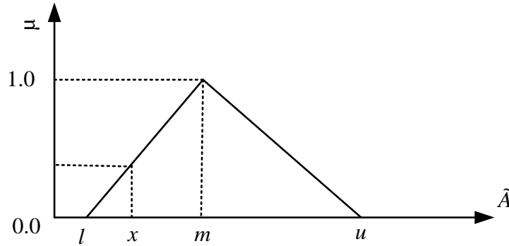
Figure 10. Representation of triangular fuzzy number (TFN) with basis denoted as (l, m, u) .
