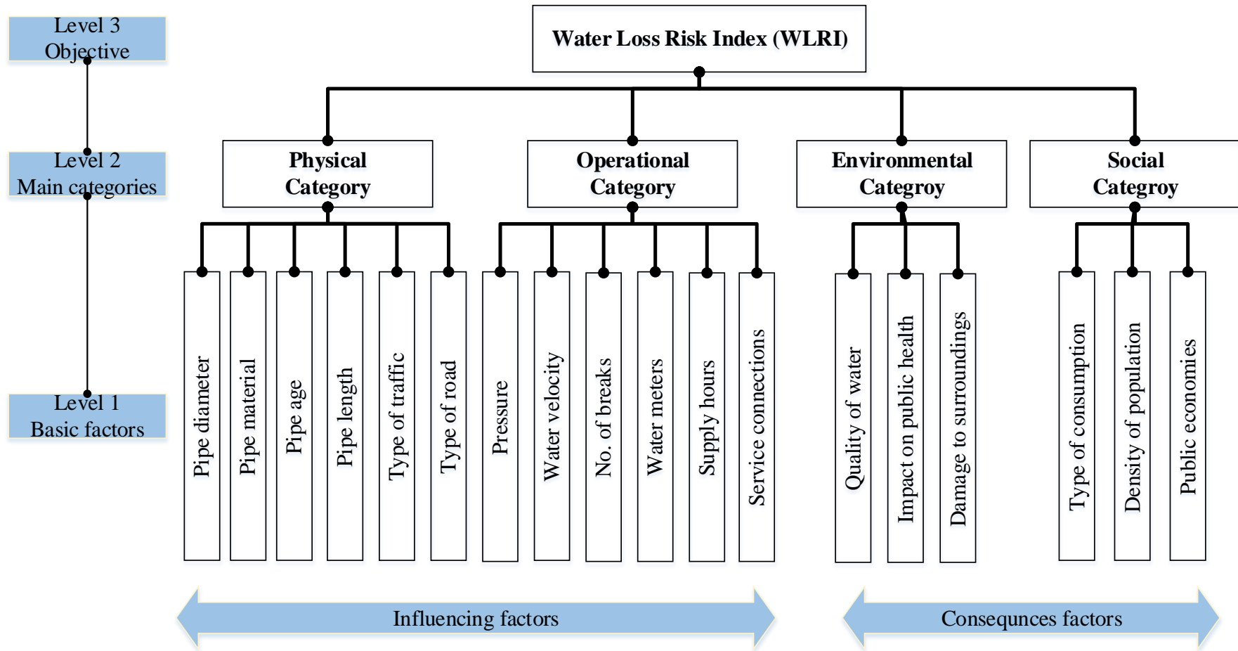
Figure 14. Hierarchical structure of contributing factors to water loss risk index (WLRI) in water distribution network
