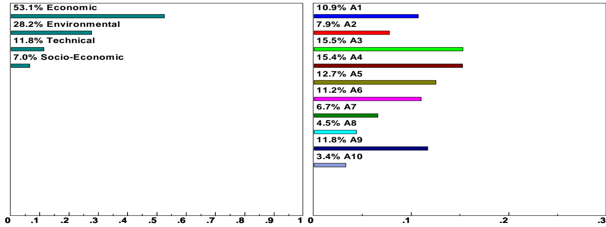
Figure E8 | Dynamic sensitivity analysis for socio-economic criterion – minimum limit of stability interval.
