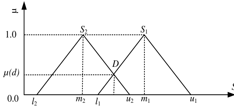
Figure 11. Illustration of intersection between two TFN numbers.
