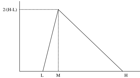
Figure 16. Triangular distribution probability density function.
