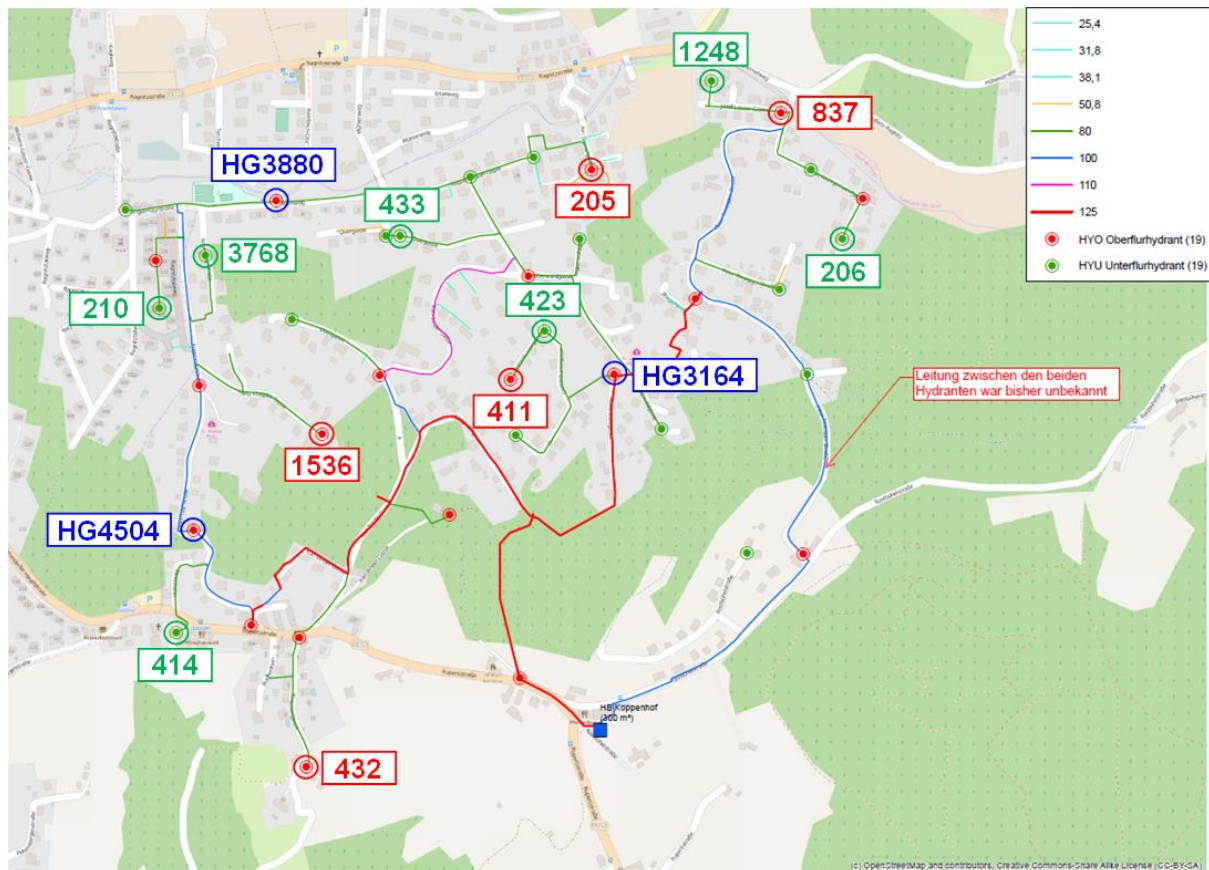
Figure 3.2: Overview map of the area (Hart close to Graz/Ragnitz) (Institute of Urban Water Management and Landscape Water Engineering/ Graz University of Technology - adapted, 2015)
