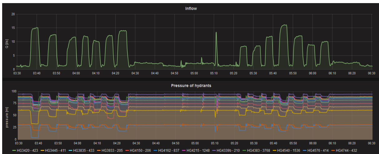
Figure 4.1: Night measurements
