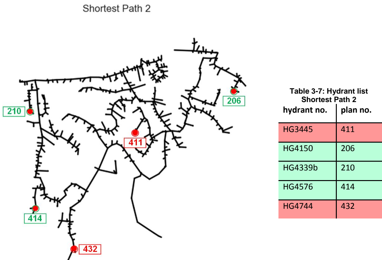
Figure 3.9: Sensor placement Shortest Path 2 (De Schaezen, et al., 2000)
