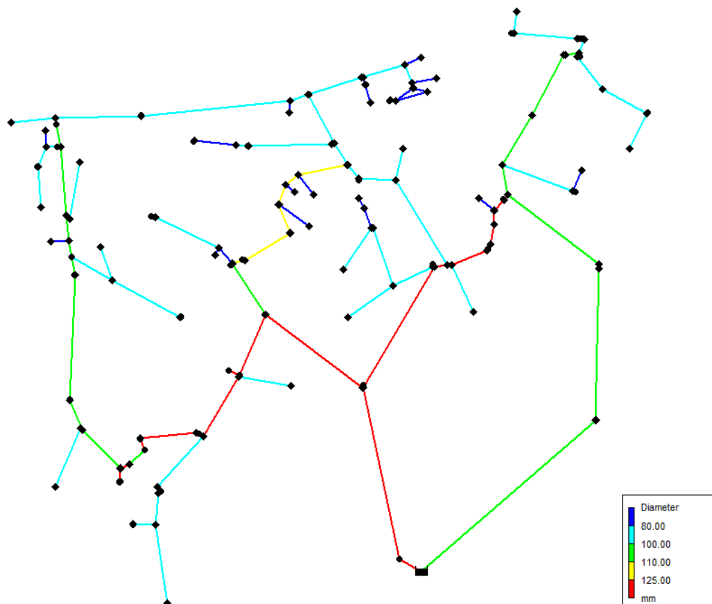
Figure 3.3: EPANET model
