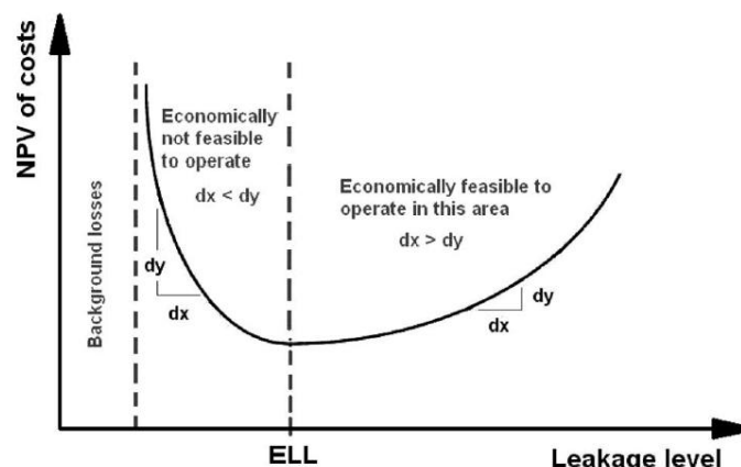
Figure 1.6: Economic level of leakage (Puust, et al., 2010)
