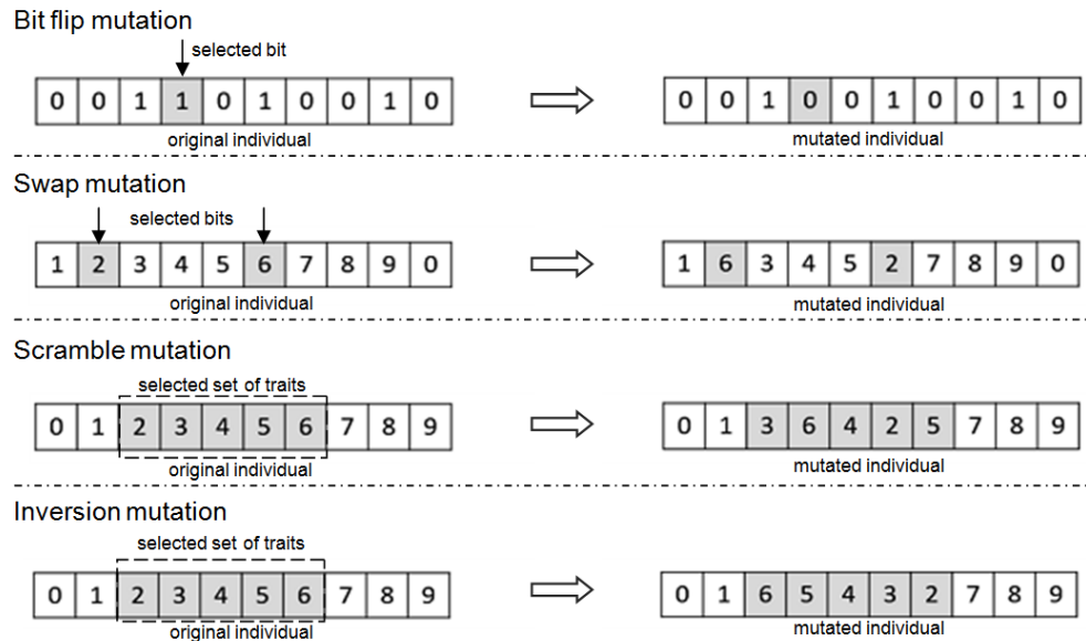
Figure 2.5: GA – bit flip mutation, swap mutation, scramble mutation and inversion mutation (Tutorialspoint)
