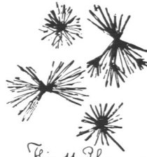
Fig. 11. Phanodorm-Thallium
