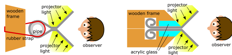
Figure 2.24: Old design on the left, with a single large frame. New design on the right, each side can easily be separated, e.g. for transport or maintenance.
