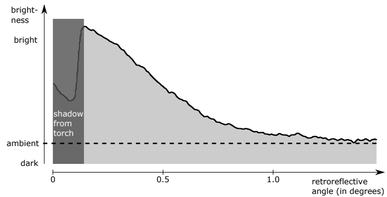
Figure 2.42: To get an idea on the angle dependent reflectivity, a photo of a light beam reflection from the retro reflective material was taken. The scan line shows the small reflection angle. On the left, the shadow of the light source hides the brightness. Note that the camera response curve is not calibrated.
