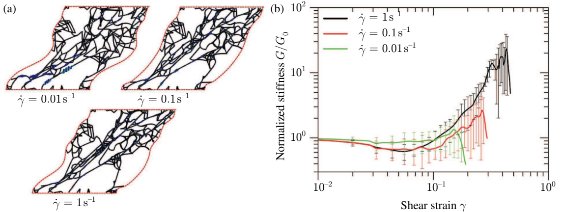
Figure 1.12: Influence of the shear rate ( \dot{\gamma} = 0.01, 0.1, 1 \text{ s}^{-1} ) on cross-link rupture. (a) Deformed network configurations at \gamma = 0.5 . (b) Shear modulus G normalized by the initial shear modulus G_0 versus shear strain \gamma for 25 network realizations and stochastic bond dissociation. Adapted from [96].
