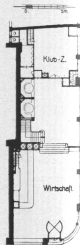
Abb. 765. Restaurant Bagenerhof, Erdgesch.
