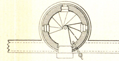
FIG. 6. Sectional Plan through Line L.M.
