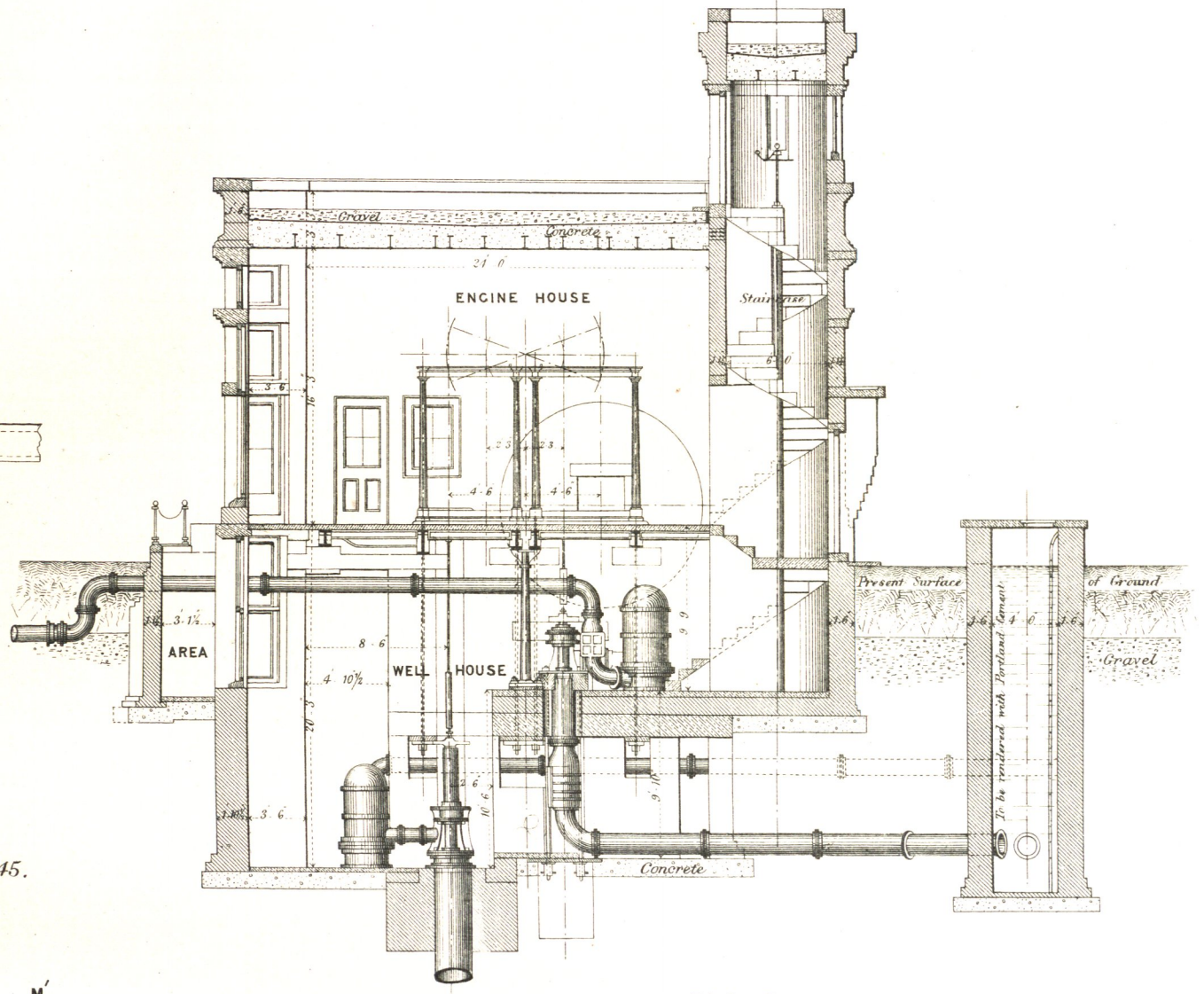
FIG. 5. Sectional Elevation through Line G.H. on Plate 45.
