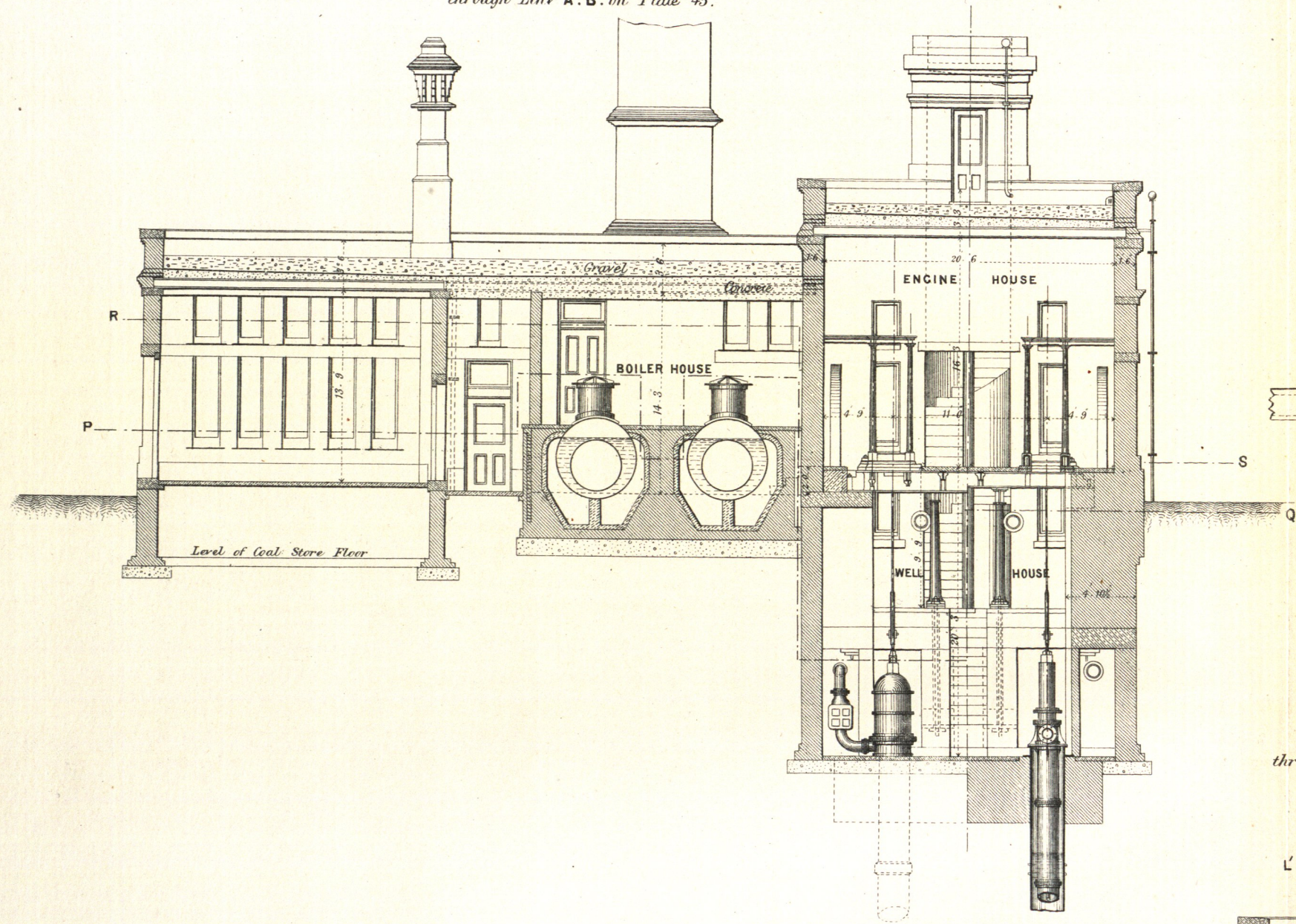
FIG. 1. Sectional Elevation through Line A.B. on Plate 45.
