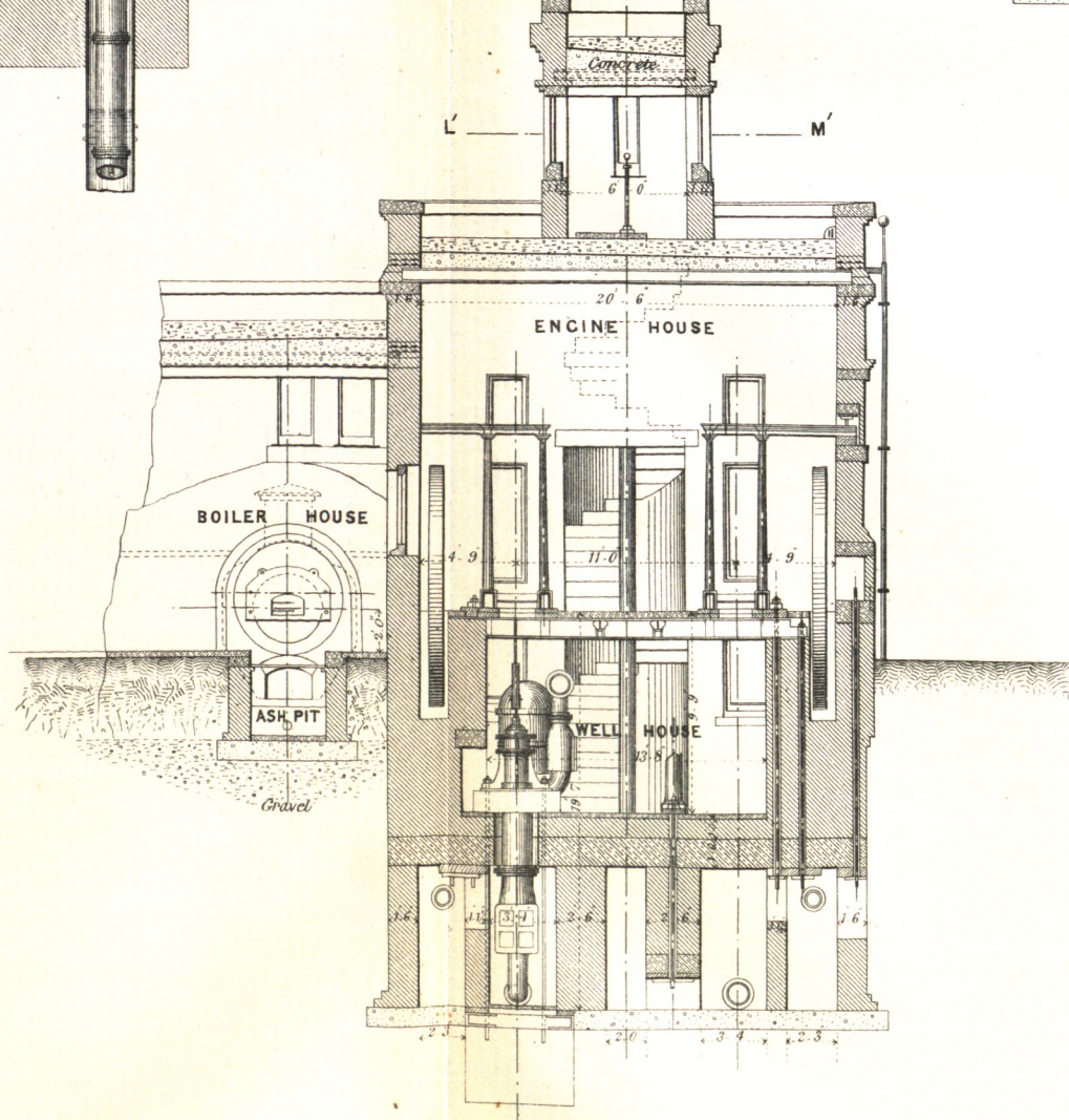
FIG. 3. Sectional Elevation through Line C.D. on Plate 45.
