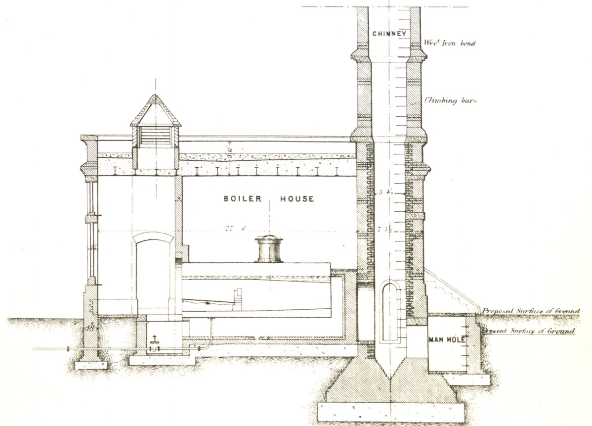
FIG. 5. Sectional Elevation through Line G.H. on Plate 45.
