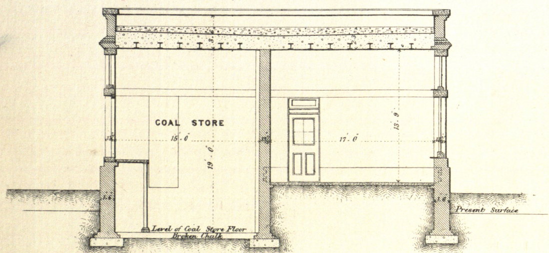
FIG. 4. Sectional Elevation through Line E.F. on Plate 45.
