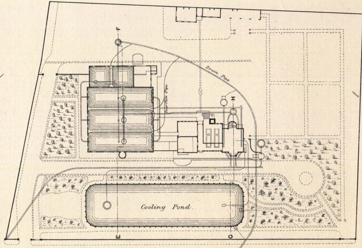
FIG. 1. General Plan.
