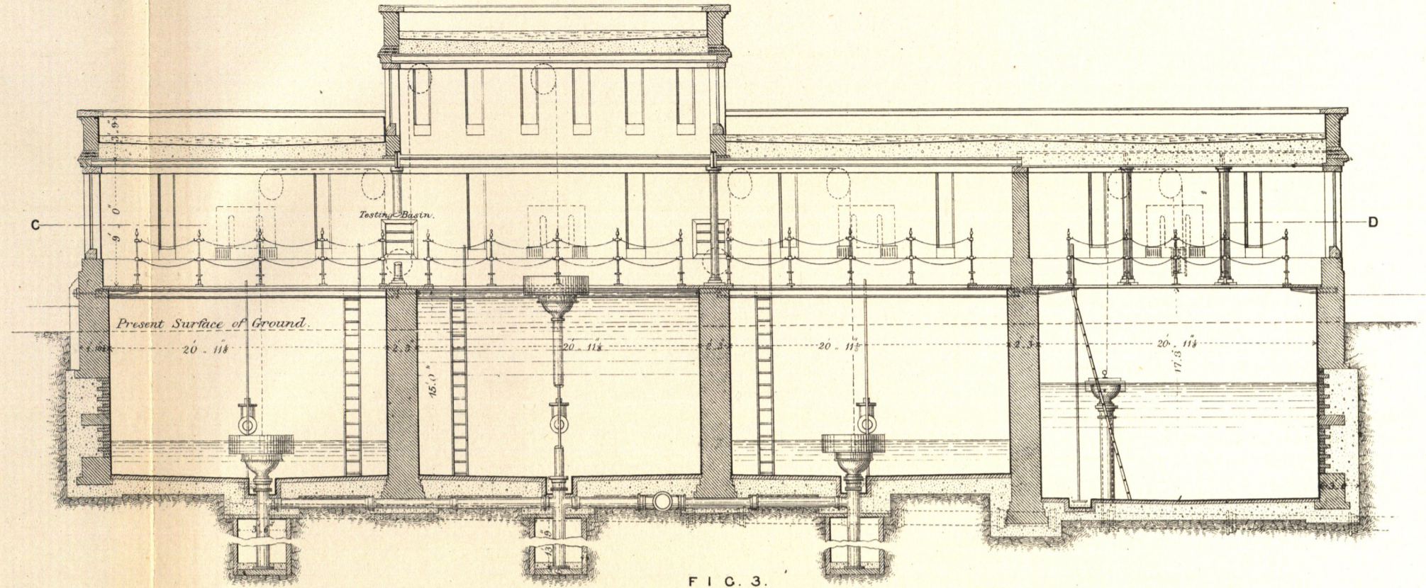
FIG. 3. Sectional Plan C. D.
