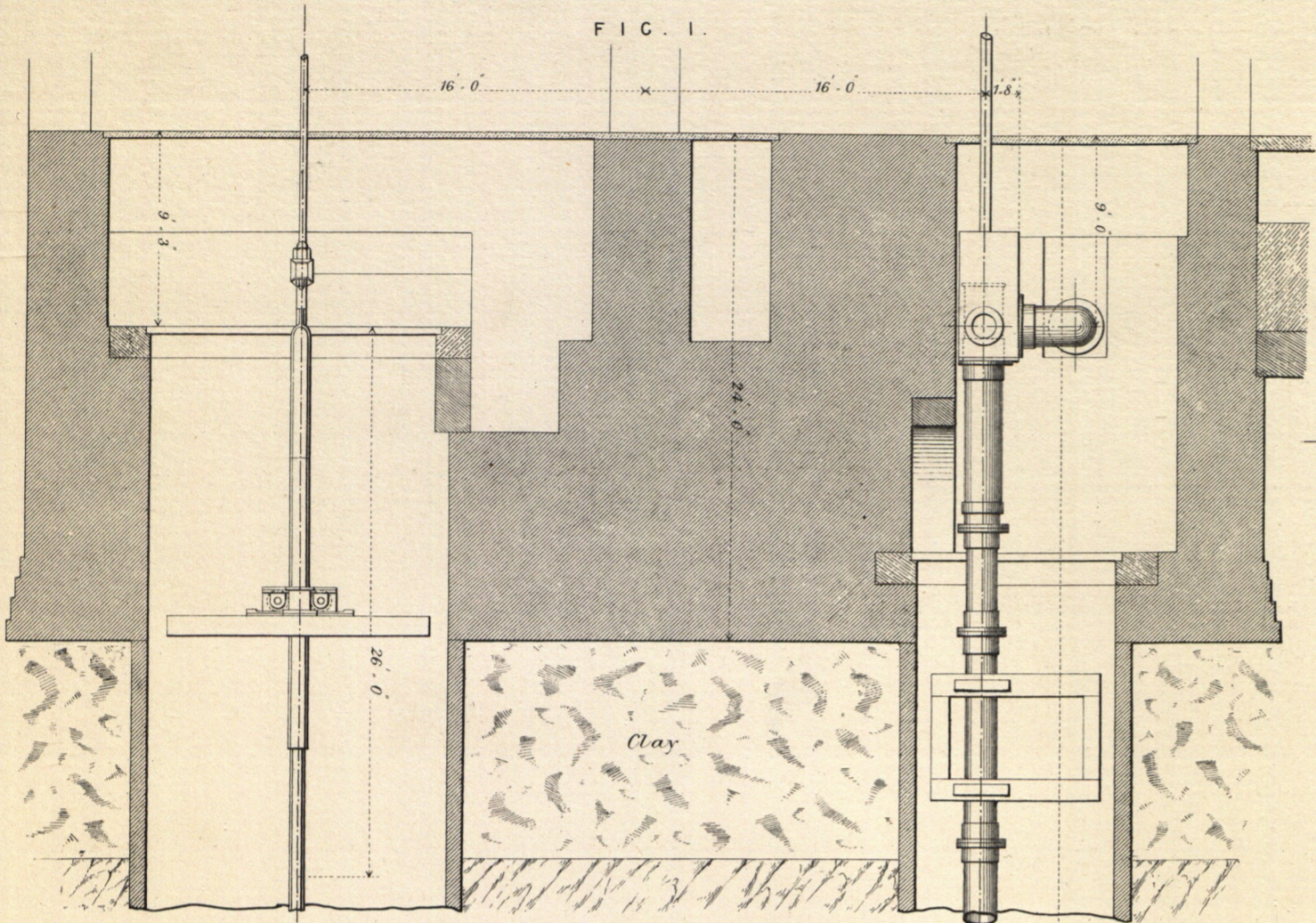
SECTIONS OF WELL AND STAPLE SHEWING PUMPS ETC.
