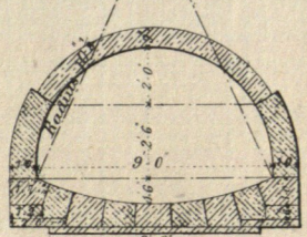
FIG. 19. Section of Waste Water Culvert
