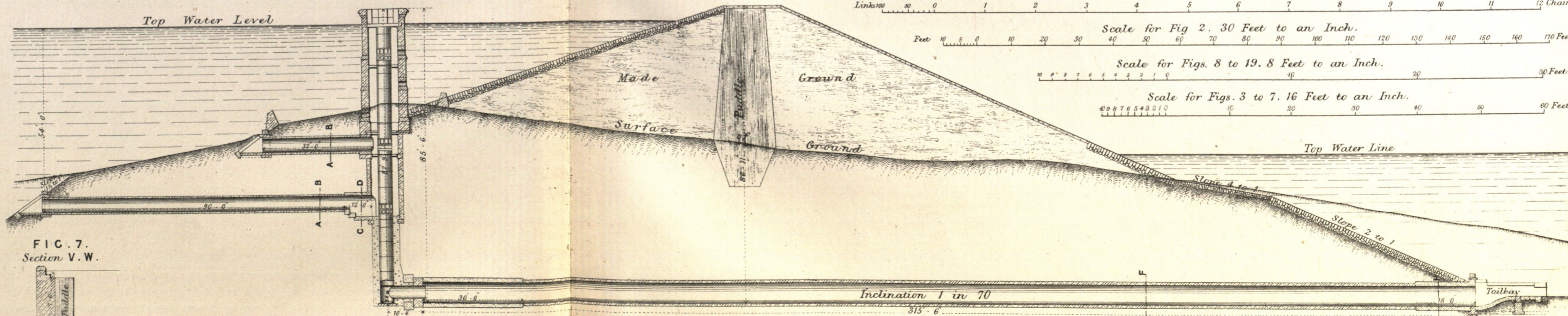
FIG. 2. Longitudinal Section of Culvert Forebay and Shaft Tower.
