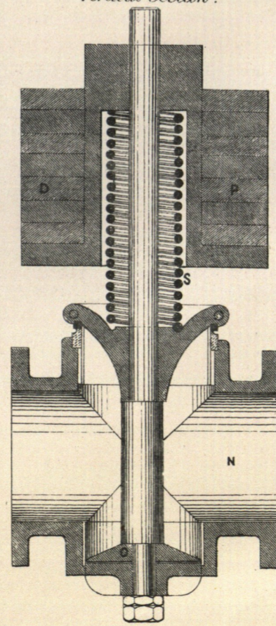
FIG. 7 Vertical Section.
