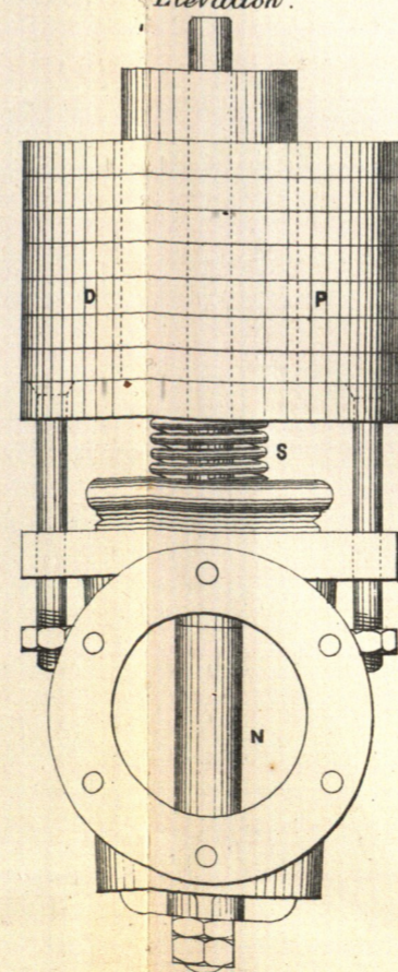
FIG. 8 Elevation.
