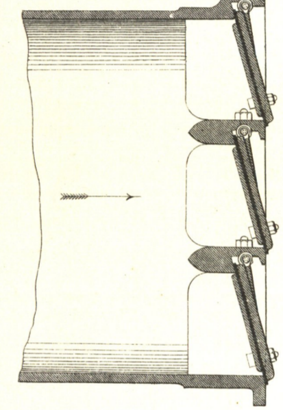
FIG. 10. Vertical Section
