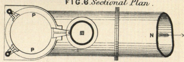
FIG. 6. Sectional Plan.
