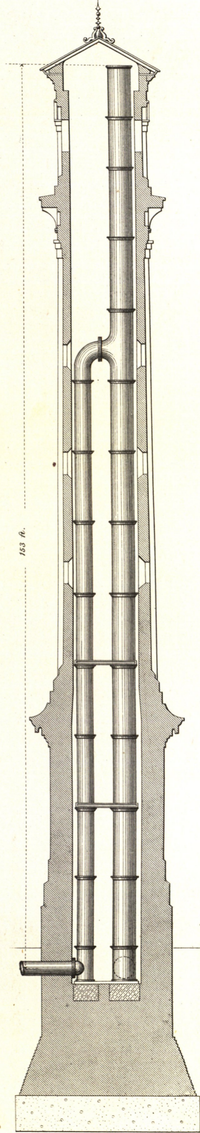
FIG. 11. Sectional Elevation.
