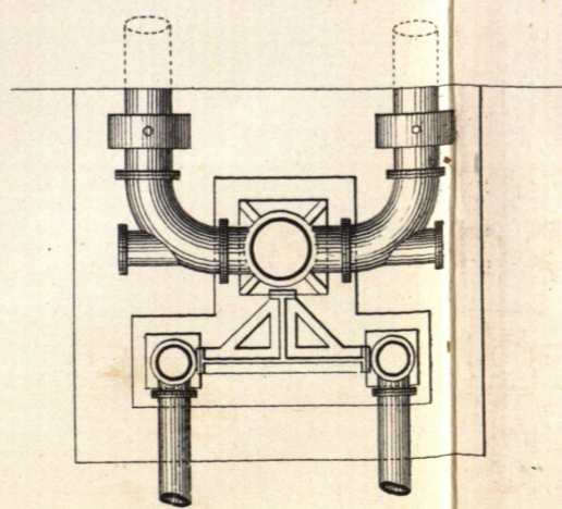
FIG. 10. Sectional Plan.
