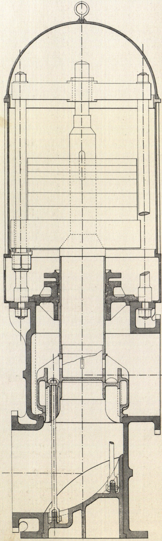
FIG. 4. Sectional Elevation.
