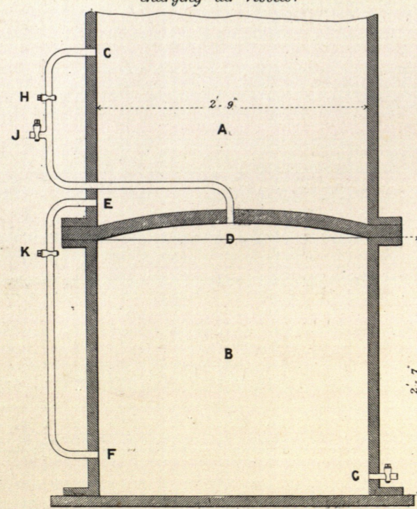
FIG. 8. Diagram shewing arrangement of charging air vessels.
