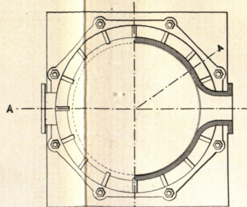
FIG. 7. Plan on Top. Sectional Plan
