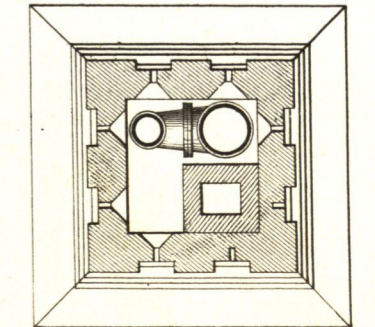
FIG. 13. Sectional Plan.
