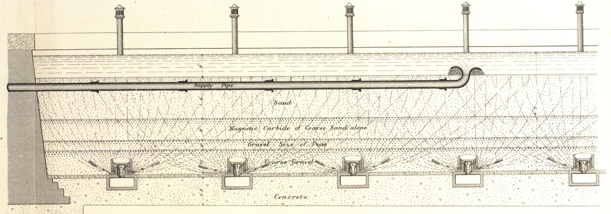
FIG. 7. Longitudinal Section of Filter Bed
