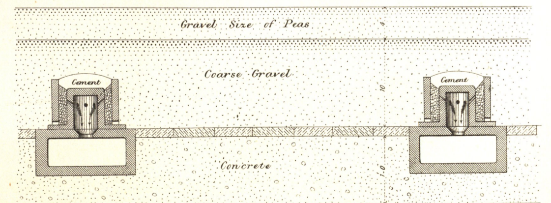
FIG. 10. Longitudinal Section of Part of Filter Bed enlarged
