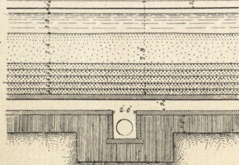
FIG. 6. Section on line C. D. enlarged
