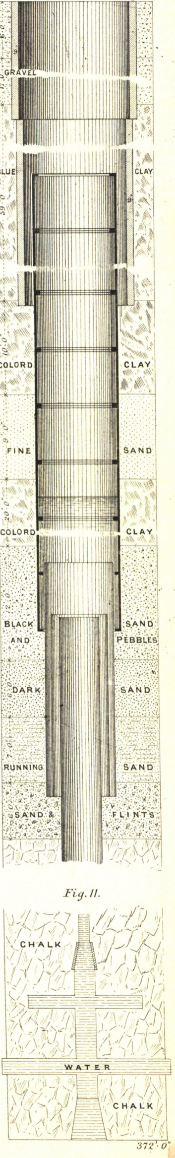
Fig. 10. HAMPSTEAD ROAD. New River Company.
