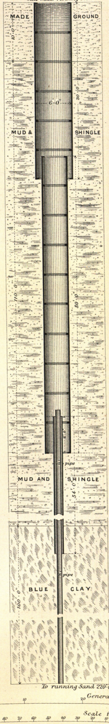
Fig. 5. SOUTHAMPTON DOCKS. Well. Salt Water running over.
