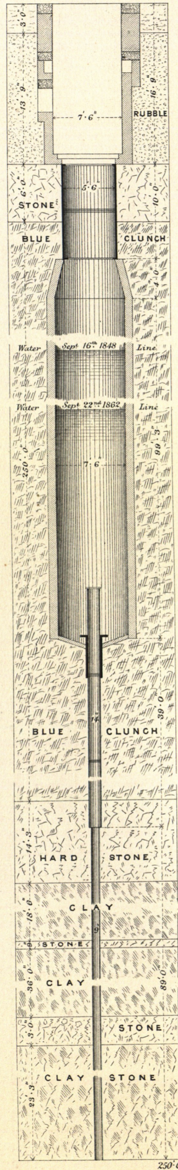
Fig. 2. NORTHAMPTON Water Works.
