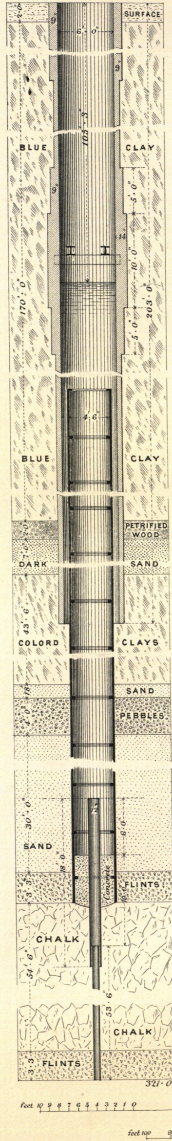
Fig. 4. KENSINGTON GARDENS. Well supplying Serpentine.
