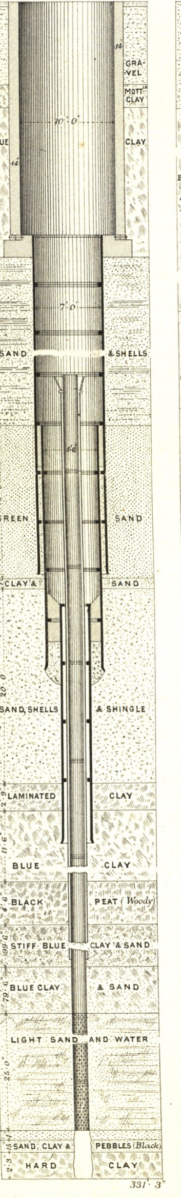
Fig. 9. GOSPORT Waterworks
