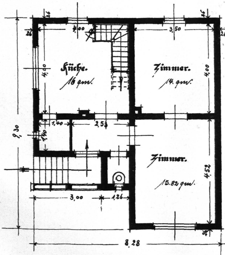
Erdgeschoss.
