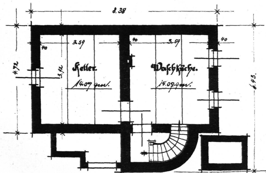
Fellergeschoss.
