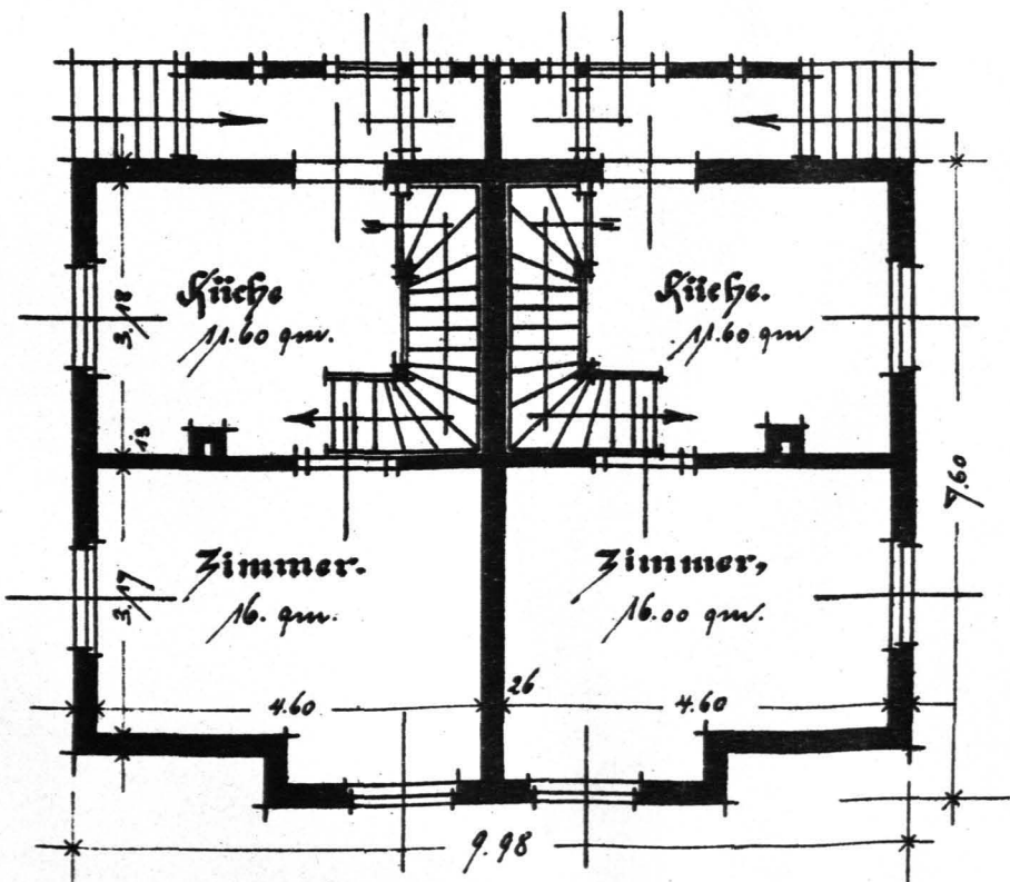
Erdgeschoss.
